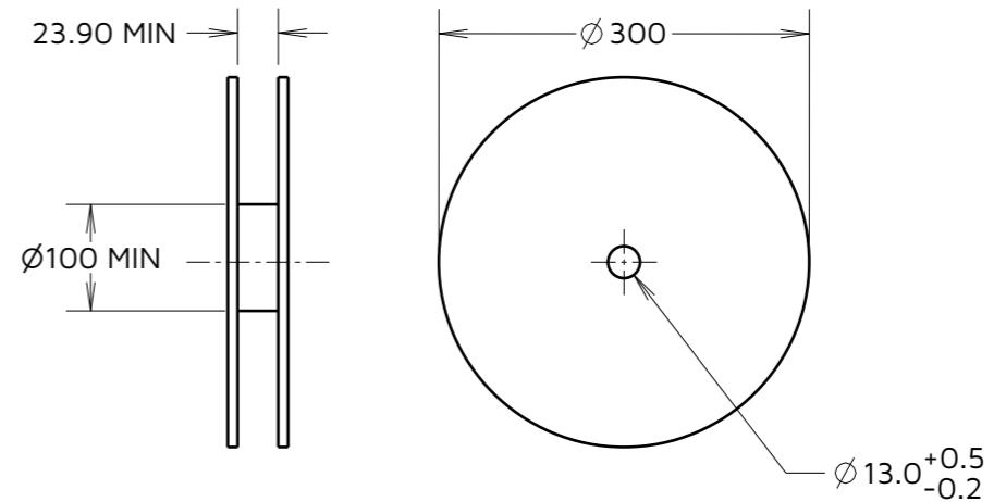
REEL DETAILS
